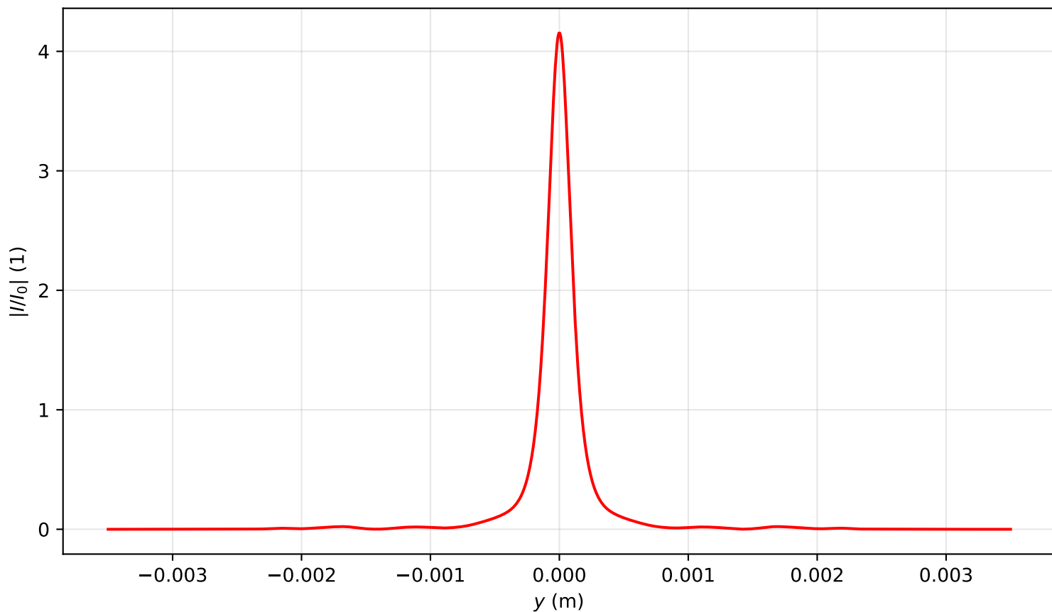
Intensity profile I(x=0, y, z=2.627)/I_0 , \text{Pin}=3.0\text{Pcr} , artificial time
